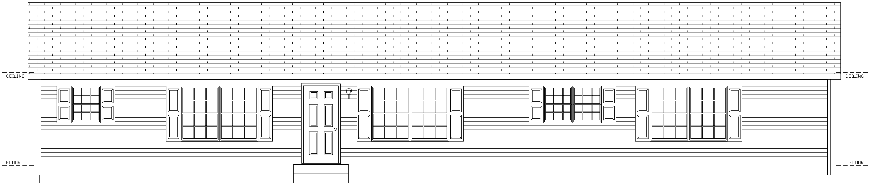
FRONT ELEVATION
