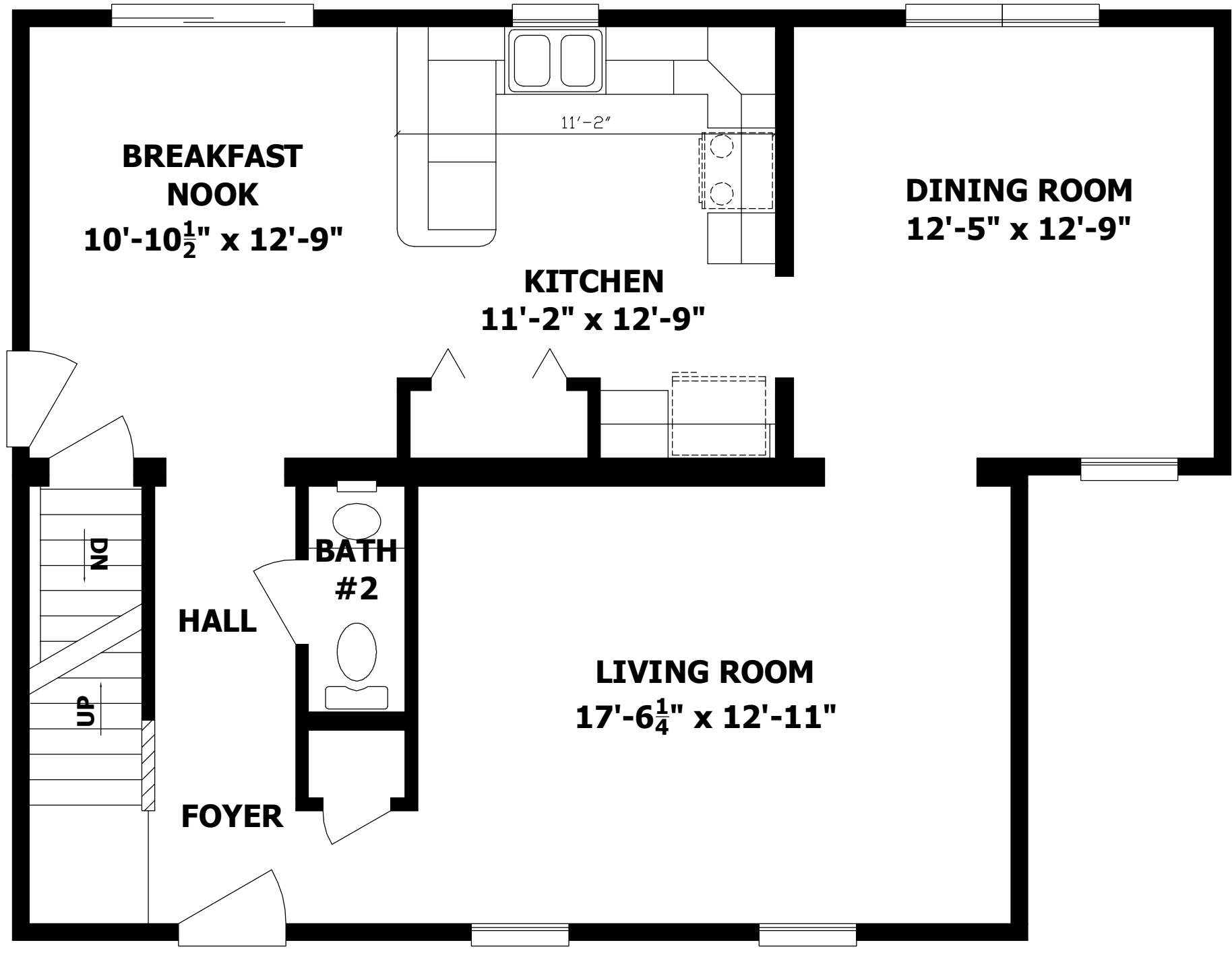
2836 TWO STORY FIRST FLOOR PLAN 907 SQ. FT. TOTAL
