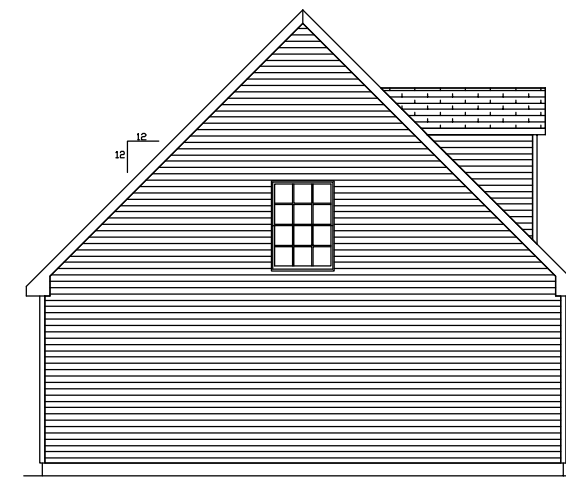
LEFT ELEVATION
