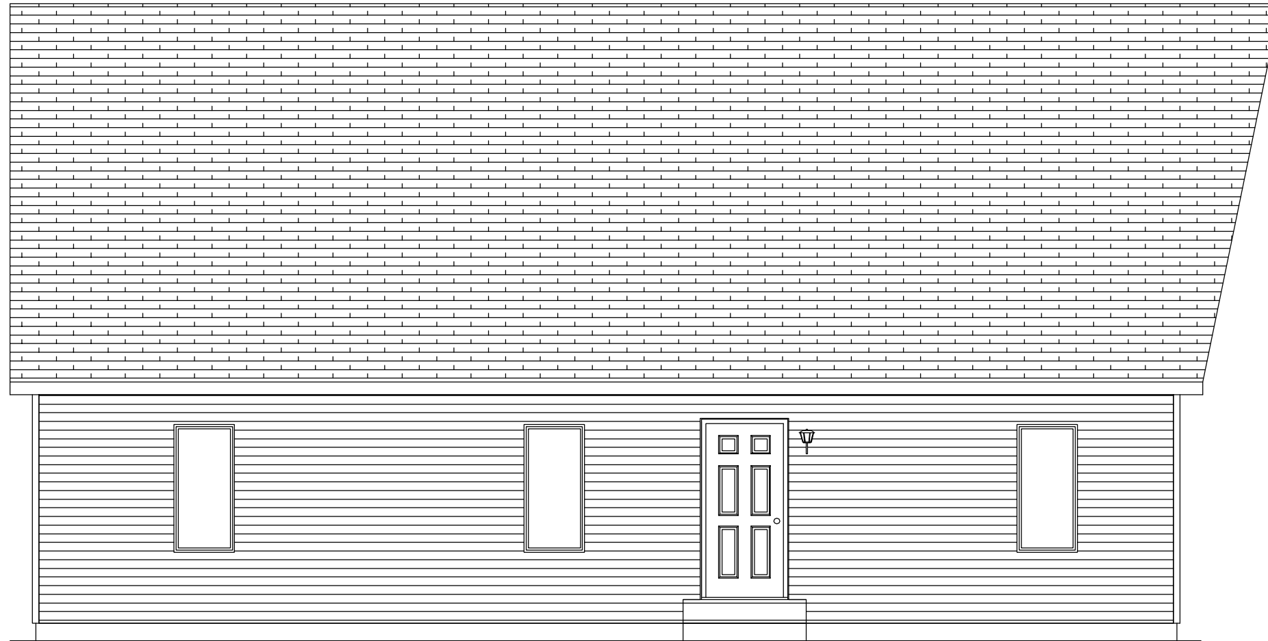
FRONT ELEVATION
