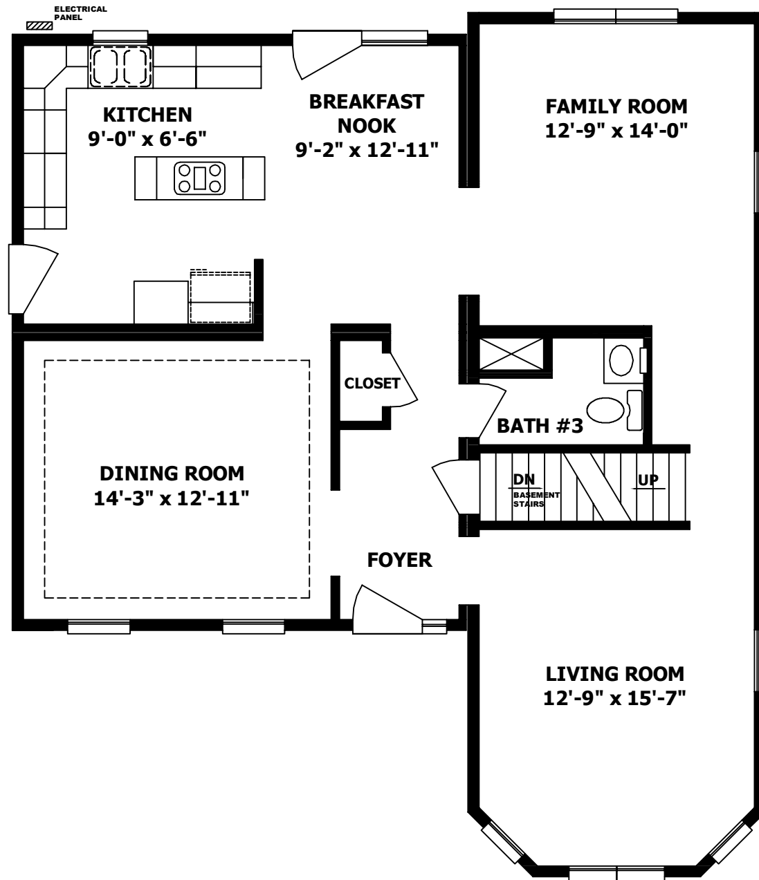
3540 TWO STORY FIRST FLOOR PLAN 1050 SQ. FT. FIRST FLOOR
