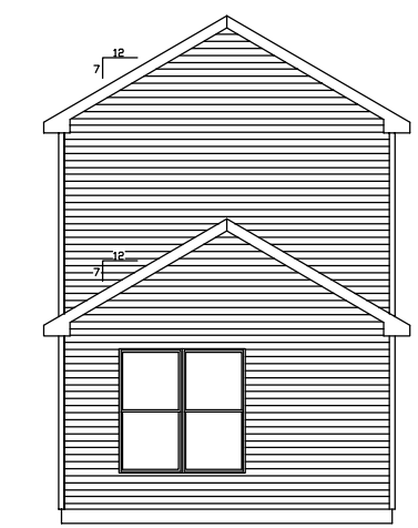
LEFT ELEVATION
